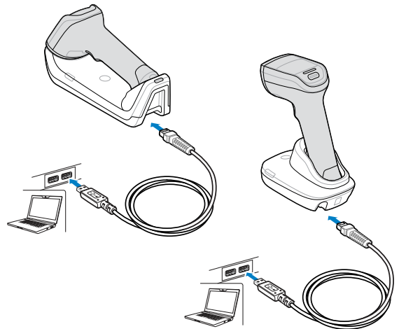
Cordless DS8288/DS8288R USB Connection
