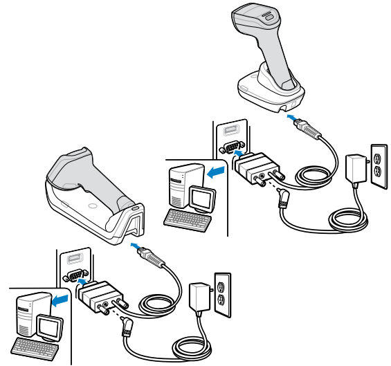
Cordless DS8288/R RS-232 Connection
